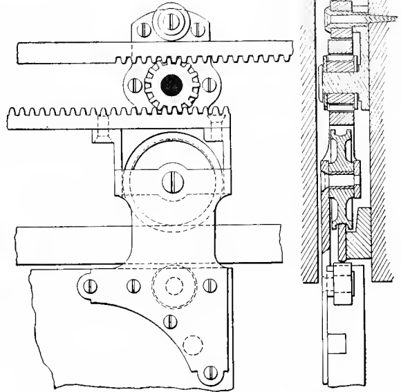
Fig. 2844. Side Elevation. Fig. 2845. Cross Section DETAILS OF DOUBLE SLIDING-DOOR FIXTURE.
